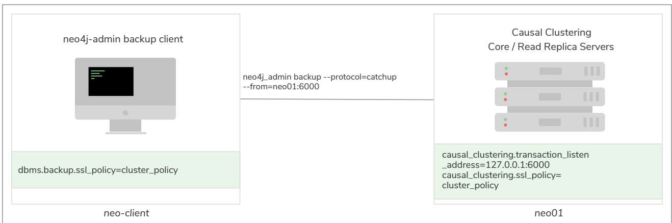
Figure 4. Settings and arguments for causal_clustering.ssl_policy
