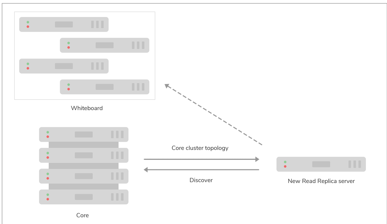
Figure 7. All Read Replicas registered with shared whiteboard.
