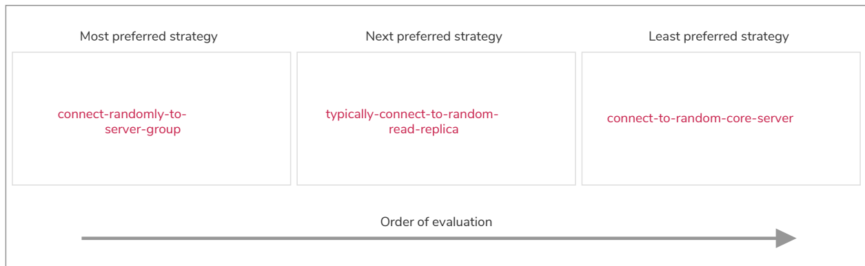
Figure 16. The first satisfactory response from a strategy will be used.
