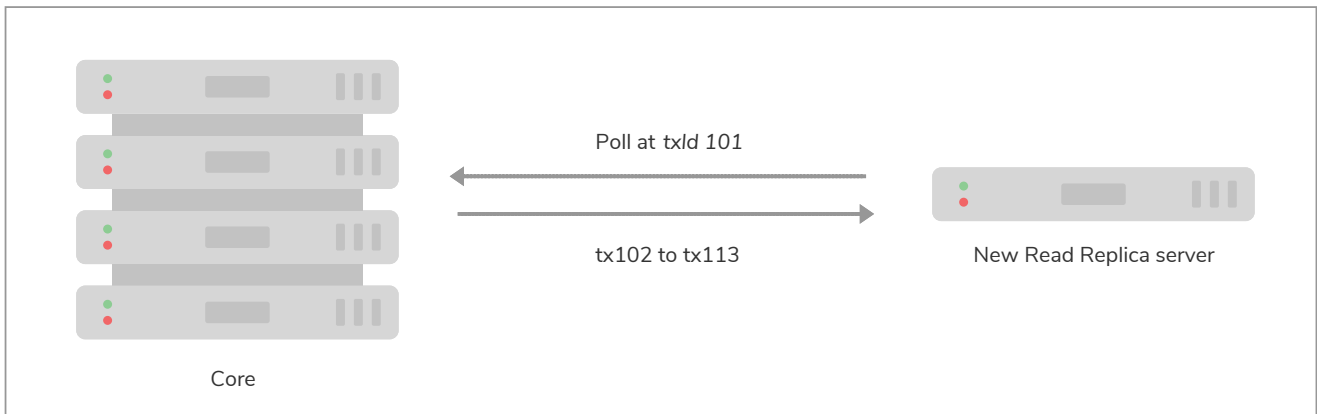
Figure 8. Transactions shipped from Core to Read Replica.
