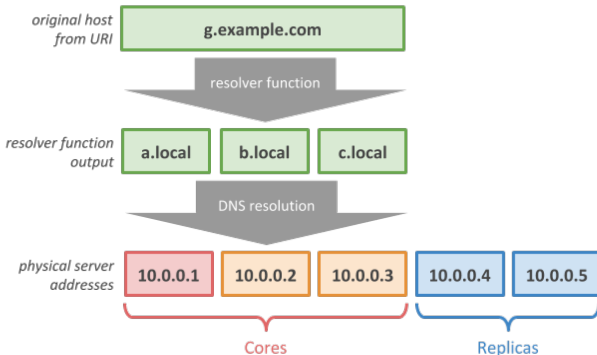
Figure 3. Initial address resolution using resolver function
