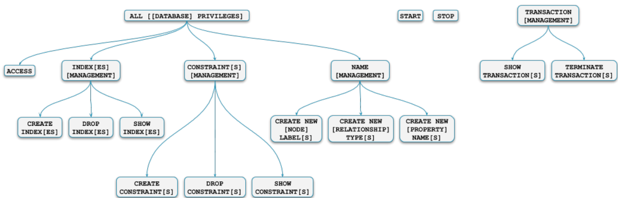
Figure 4. Database privileges hierarchy
