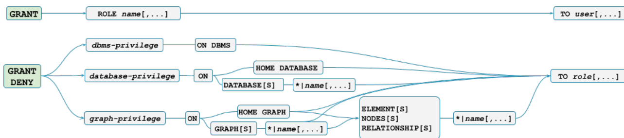
Figure 1. GRANT and DENY Syntax
