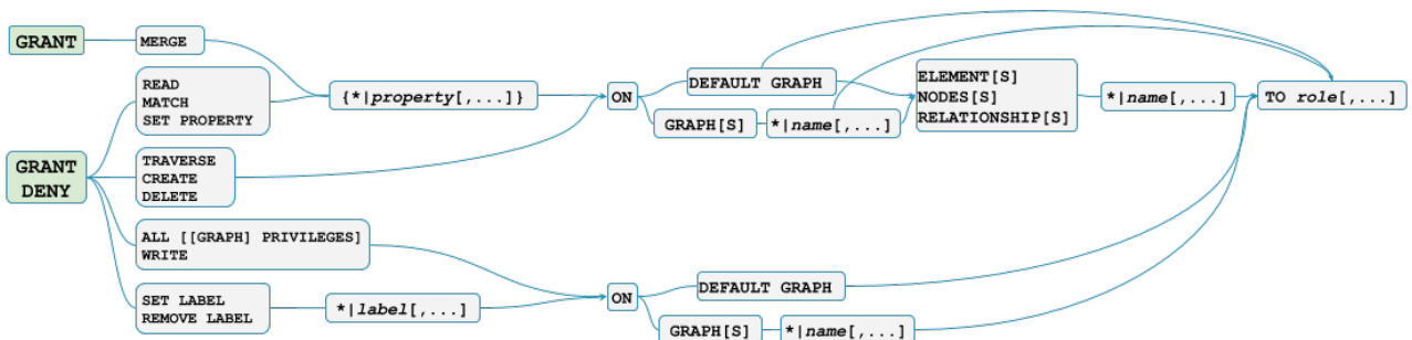
Figure 2. Syntax of GRANT and DENY Graph Privileges. The { and } are part of the syntax and not used for grouping.
