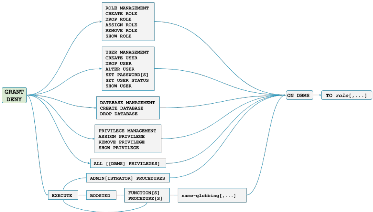
Figure 6. Syntax of GRANT and DENY DBMS Privileges
