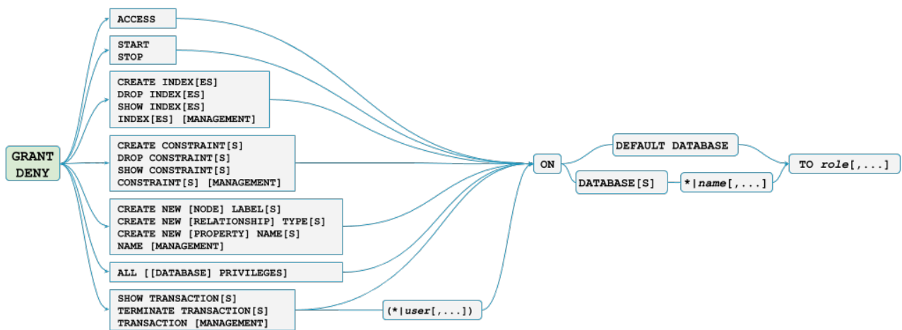
Figure 5. Syntax of GRANT and DENY Database Privileges
